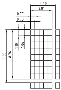
Dot's Detail Scale=3:1
